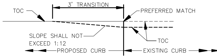
TYPICAL TRANSITION OF PROPOSED TO EXISTING TOP OF CURB
