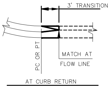
AT CURB RETURN
