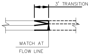
AT TANGENT SECTION
