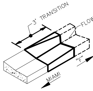
ISOMETRIC
