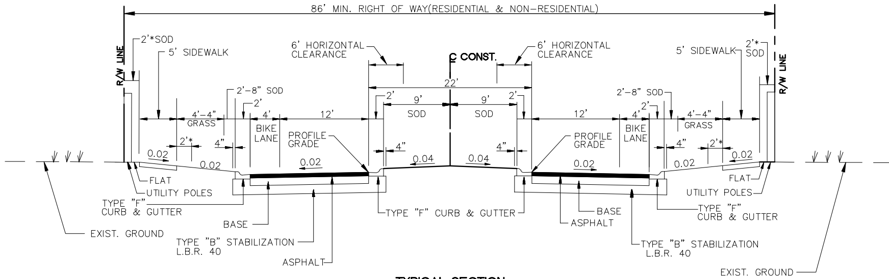
TYPICAL SECTION N.T.S. 5,000 TO 10,000 AADT
